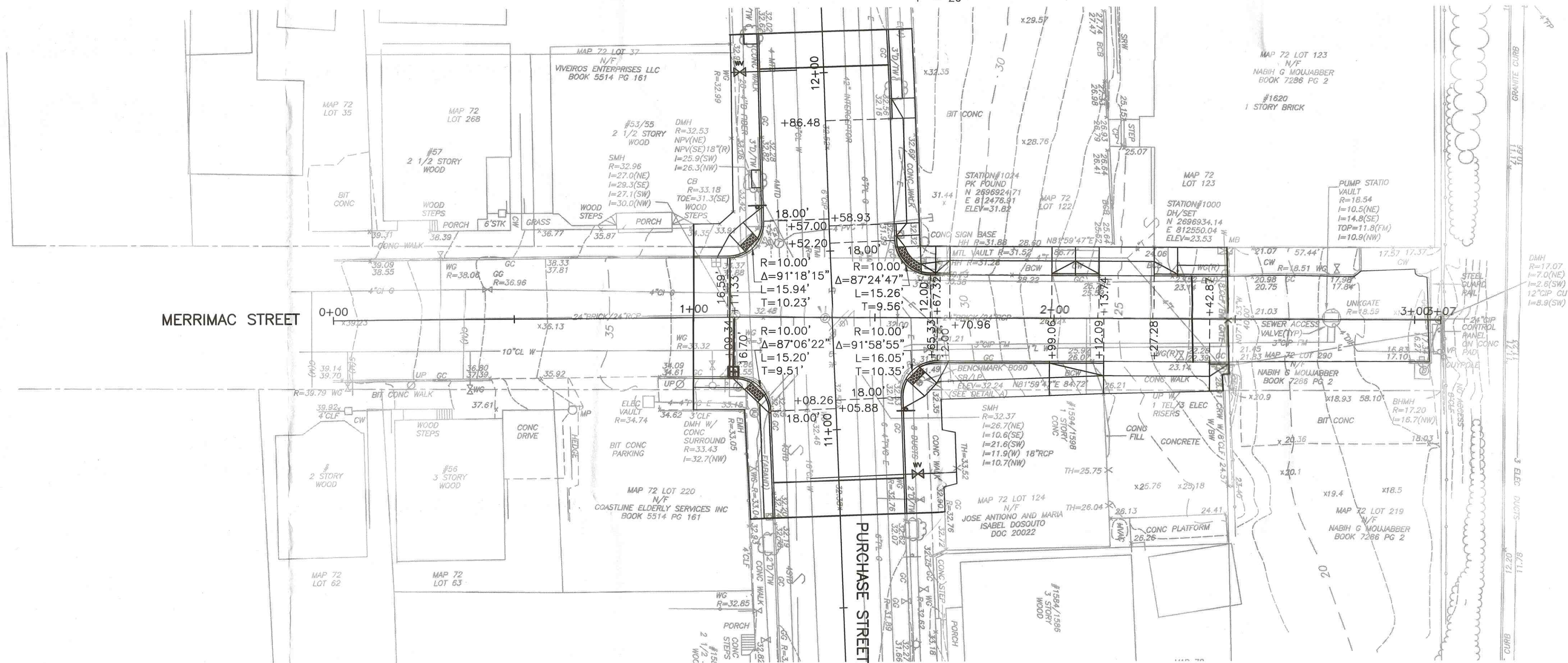
CURB TIE PLAN
