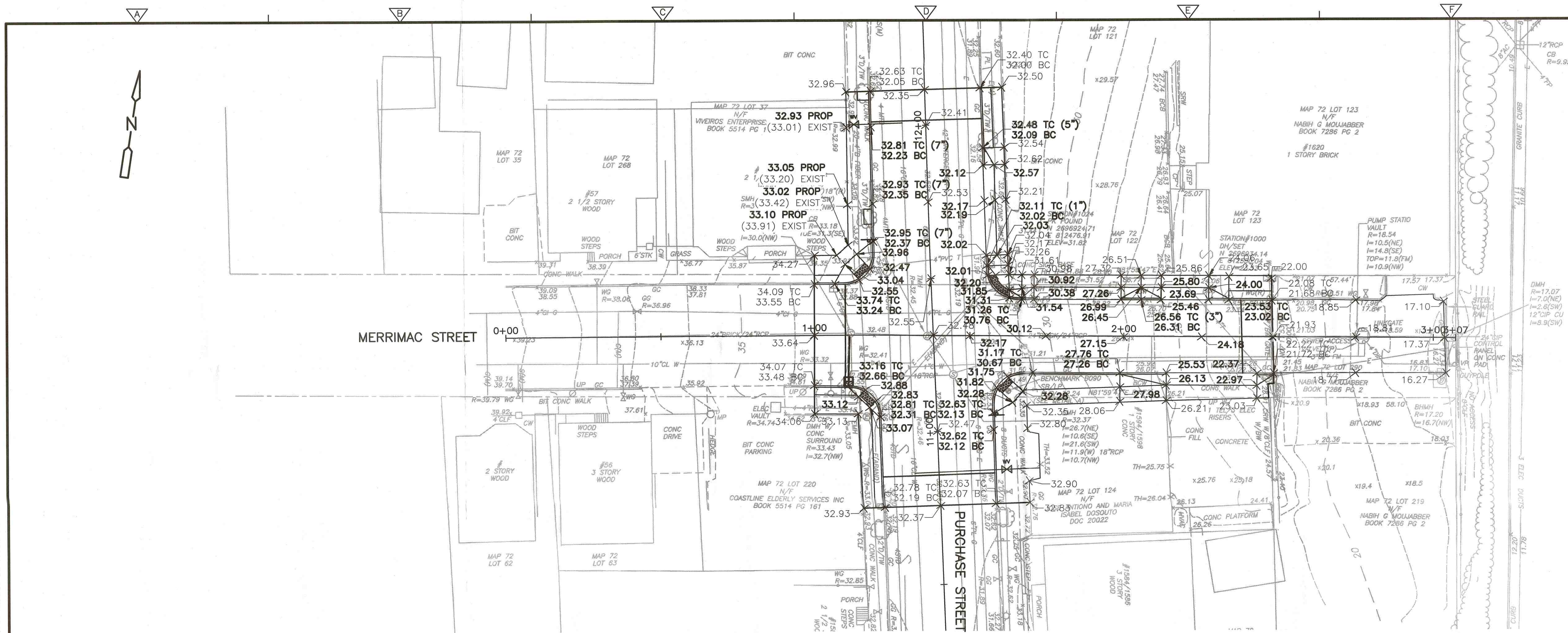
GRADING PLAN
