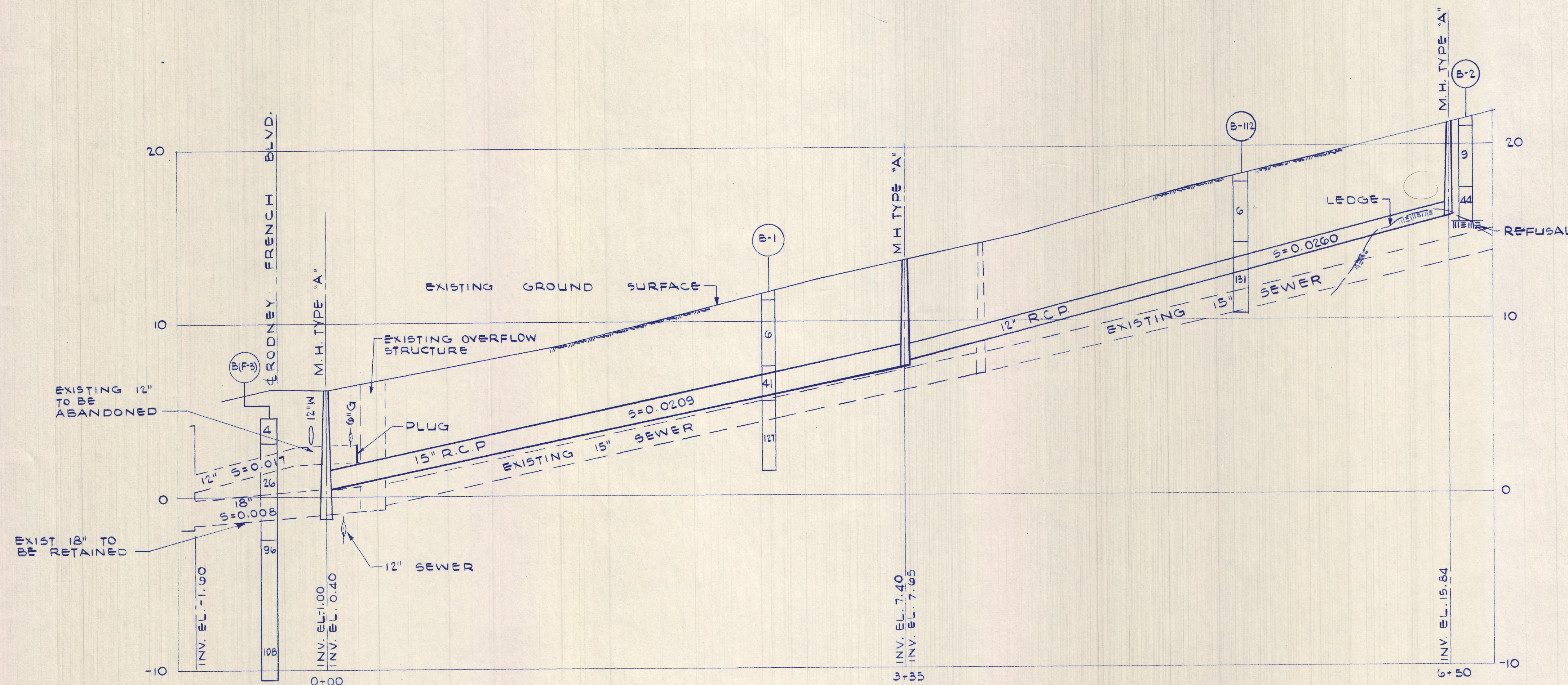
PROFILE SCALE: HOR. 1" = 40' VERT. 1" = 4'
