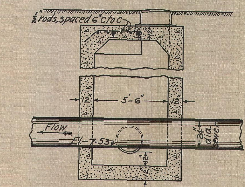
Sectional elevation. Scale: 1/4" = 1'-0"
