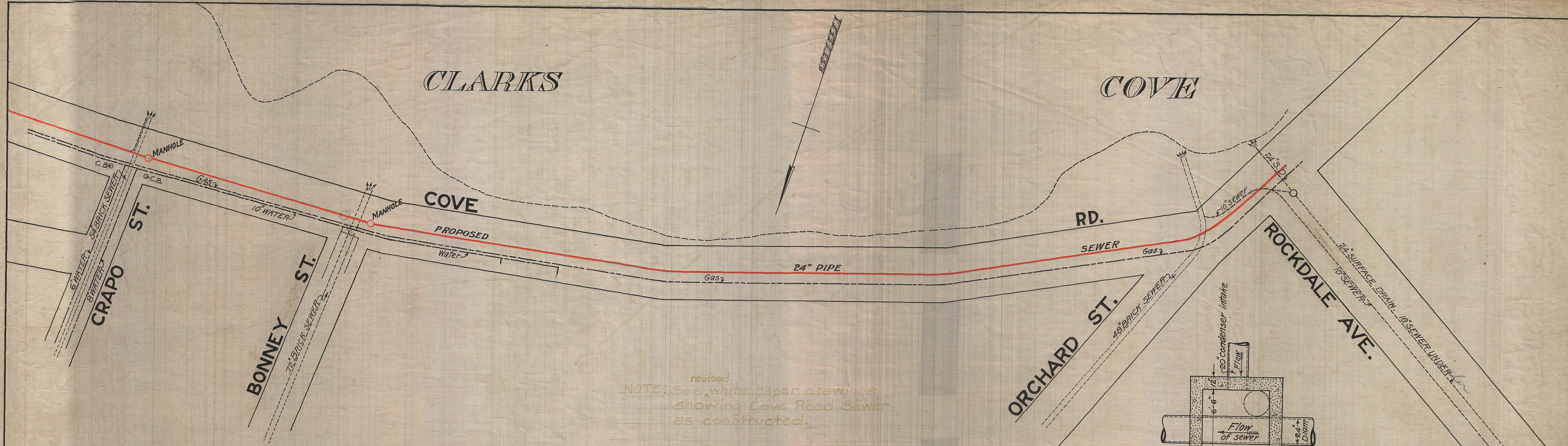
Intake Well at Sta. 10+30
