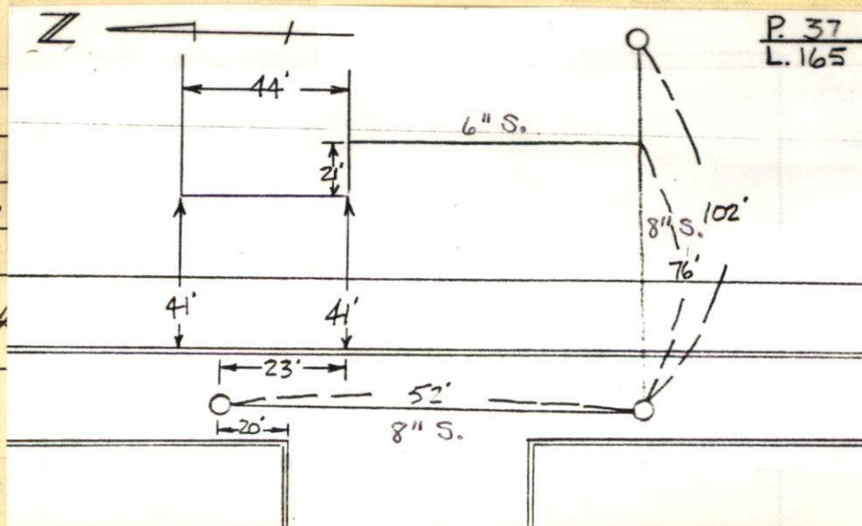
SKETCH PLAN
