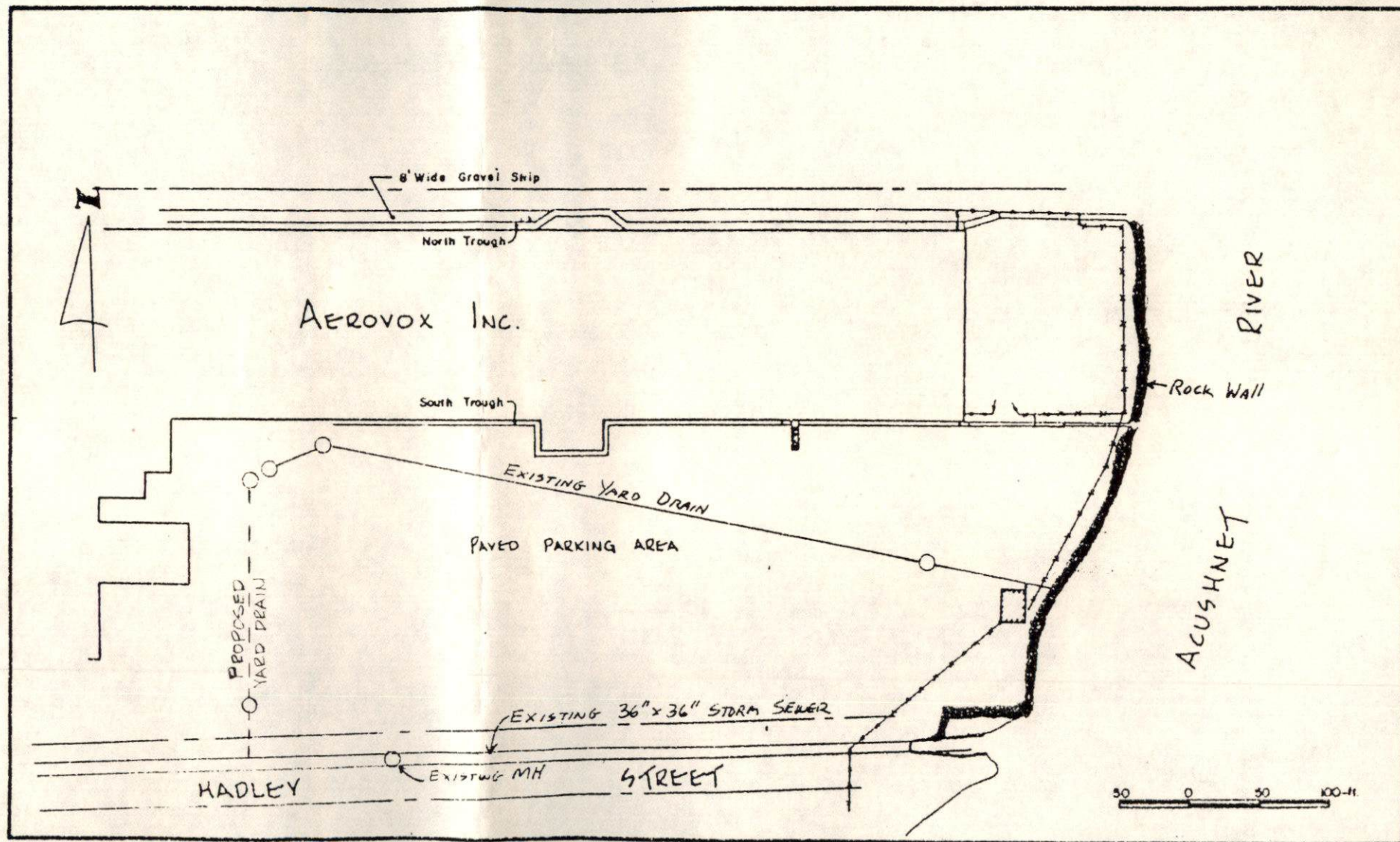
SITE PLAN SHOWING LOCATION OF PROPOSED PARKING LOT DRAINAGE SYSTEM MODIFICATIONS AT AEROVOX
