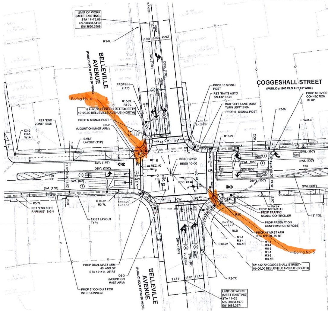
PROPOSED SIGNAL LAYOUT
