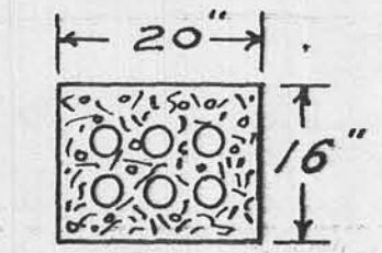
SECTION THROUGH CONDUIT 6-3/4" FIBRE DUCTS.
