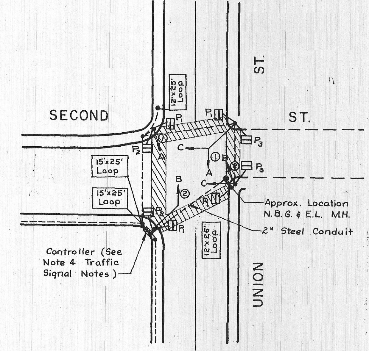
SECOND ST. - UNION ST. SCALE: 1" = 40'
