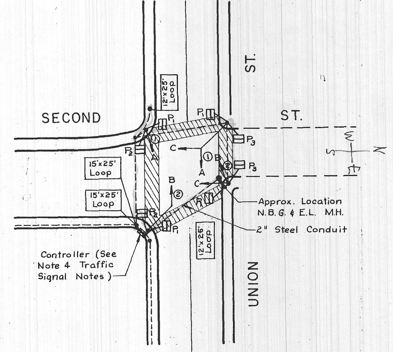
SECOND ST. - UNION ST. SCALE: 1" = 40'
