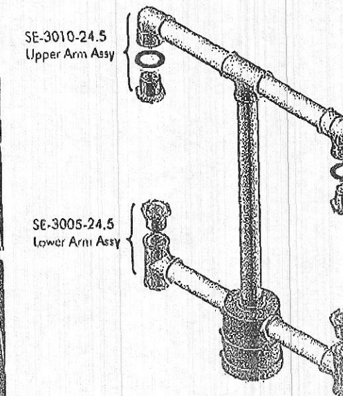
Slip Fitter Assy, 2-Way ICC Ped 24-1/2" CTC for 4-1/2" OD Pole Cast Nipple
