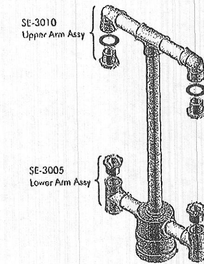
Slip Fitter Assy, 2-Way 16-1/2" CTC for 4-1/2" OD Pole Cast Nipple
