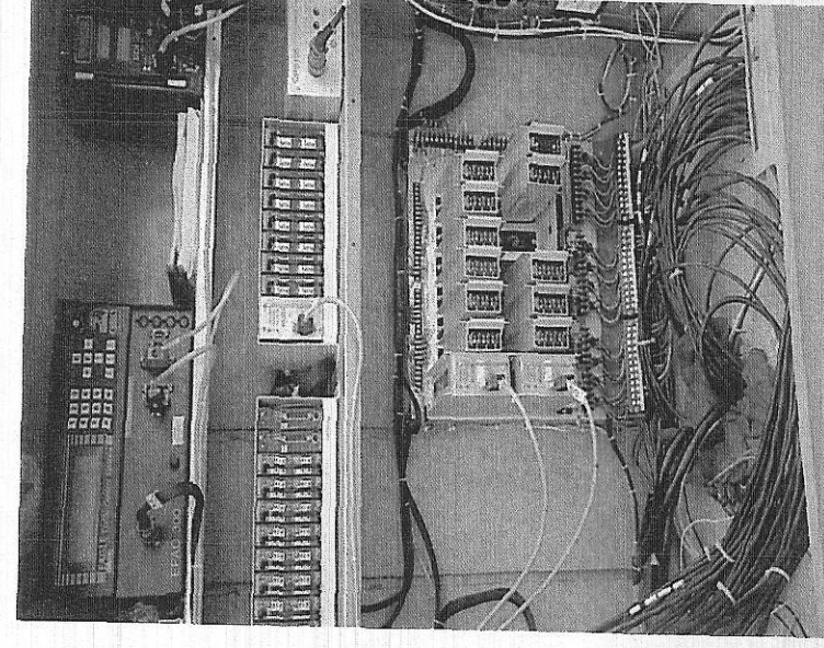
Controller cabinet located at the northeast corner of the intersection
