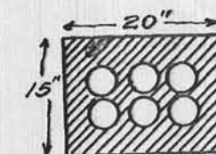
SECTION THROUGH CONDUIT 6-3 1/2" FIBRE DUCTS
