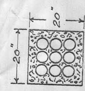
SECTION THROUGH CONDUIT ON LINE A-A 9-3\"/>
