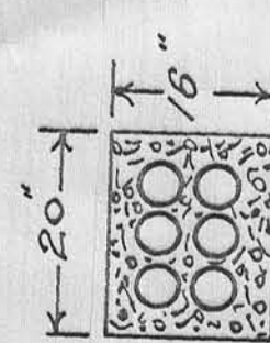
SECTION THROUGH CONDUIT. 6-3\"/>
