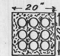
SECTION THROUGH CONDUIT.
