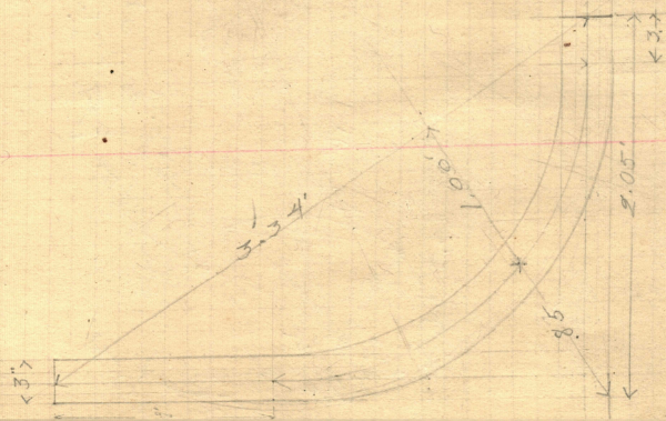
STANDARD 4 FT. 3" QUARTER BEND IRON RISER PIPE
