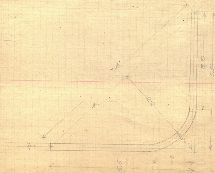
3" STANDARD 10 FT. GALVANIZED IRON BEND
